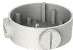
DS-1260ZJ Junction box
